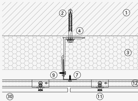
Junta vertical
