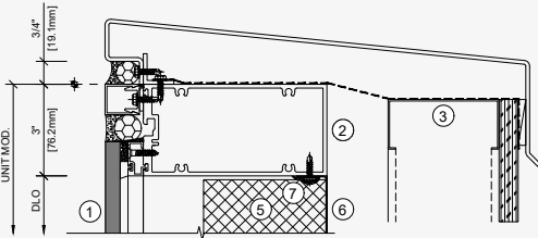
Remate Superior
