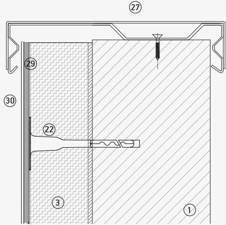
Remate superior
