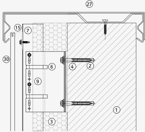
Remate superior
