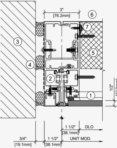
Detalle Jamba
