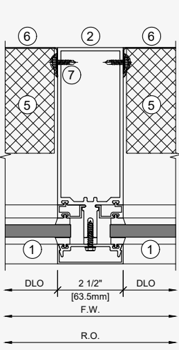
Junta Vertical
