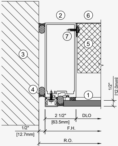
Detalle Jamba
