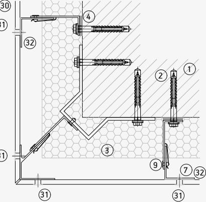
Junta vertical
