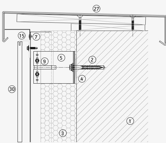
Remate superior
