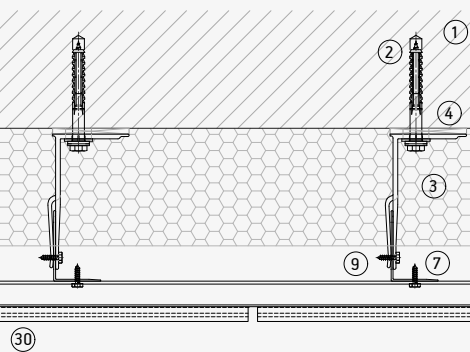
Junta vertical
