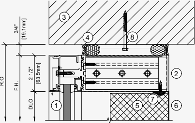
Remate Superior
