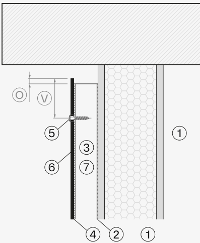
Remate superior
