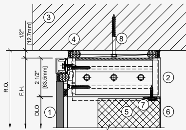
Remate Superior
