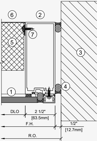
Detalle Jamba
