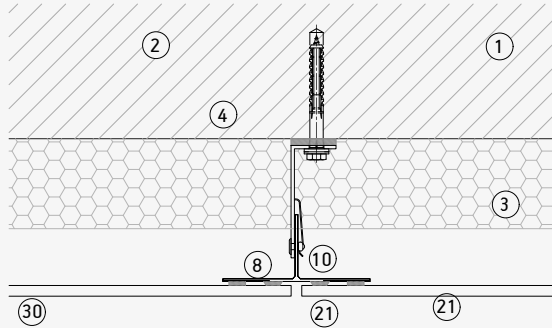
Junta vertical
