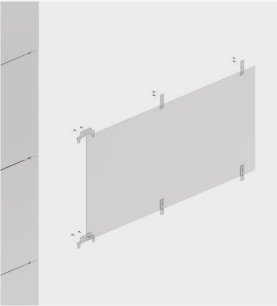
Grapas intermedias
