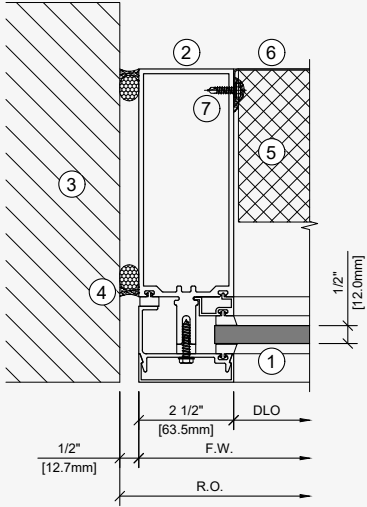
Detalle Jamba
