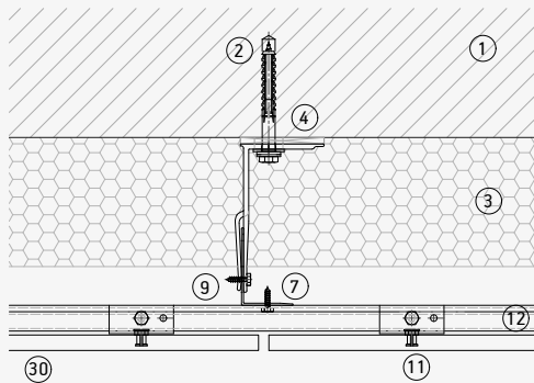
Junta vertical
