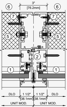
Junta Vertical
